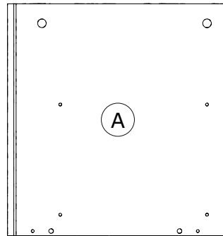
FI10211 404x385x16mm
